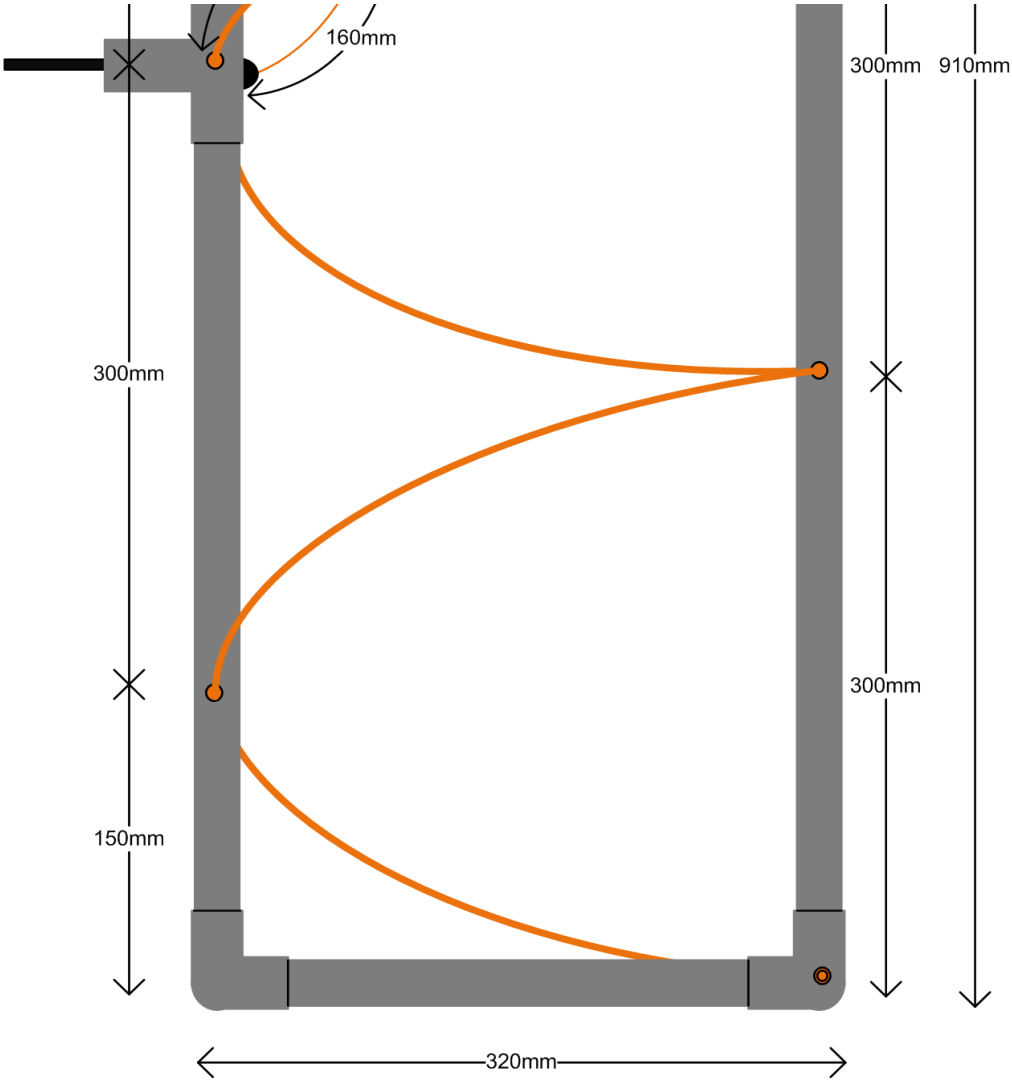
2m Mixed Mode Helix - © G8JNJ 2014
